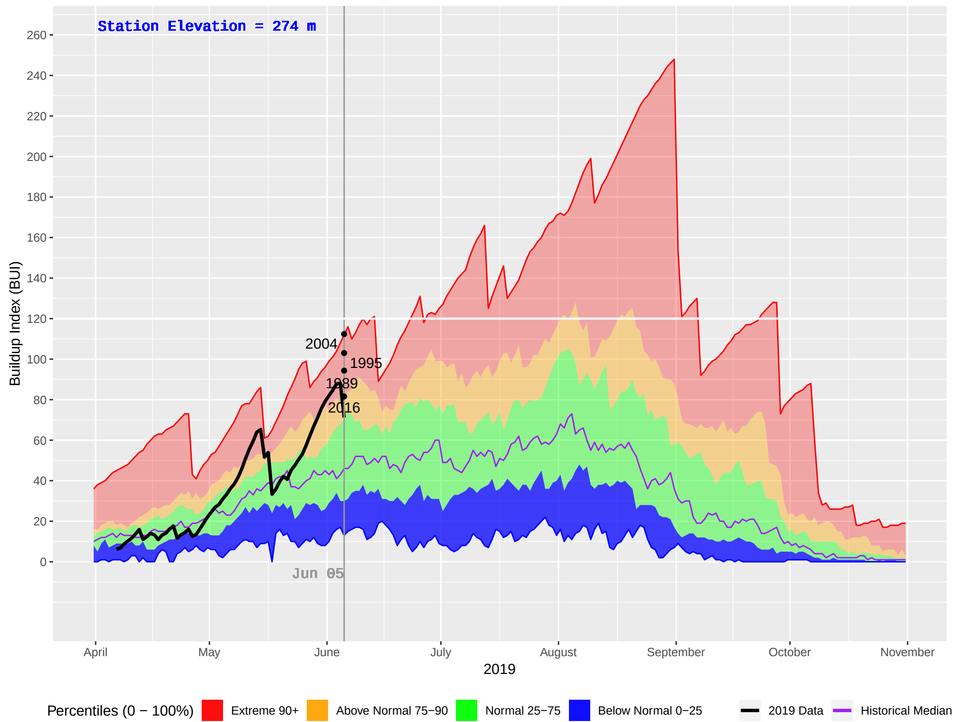
CEDARVALE (429) : Historical (1982–2018), Current (2019) Daily Buildup Index (BUI)
