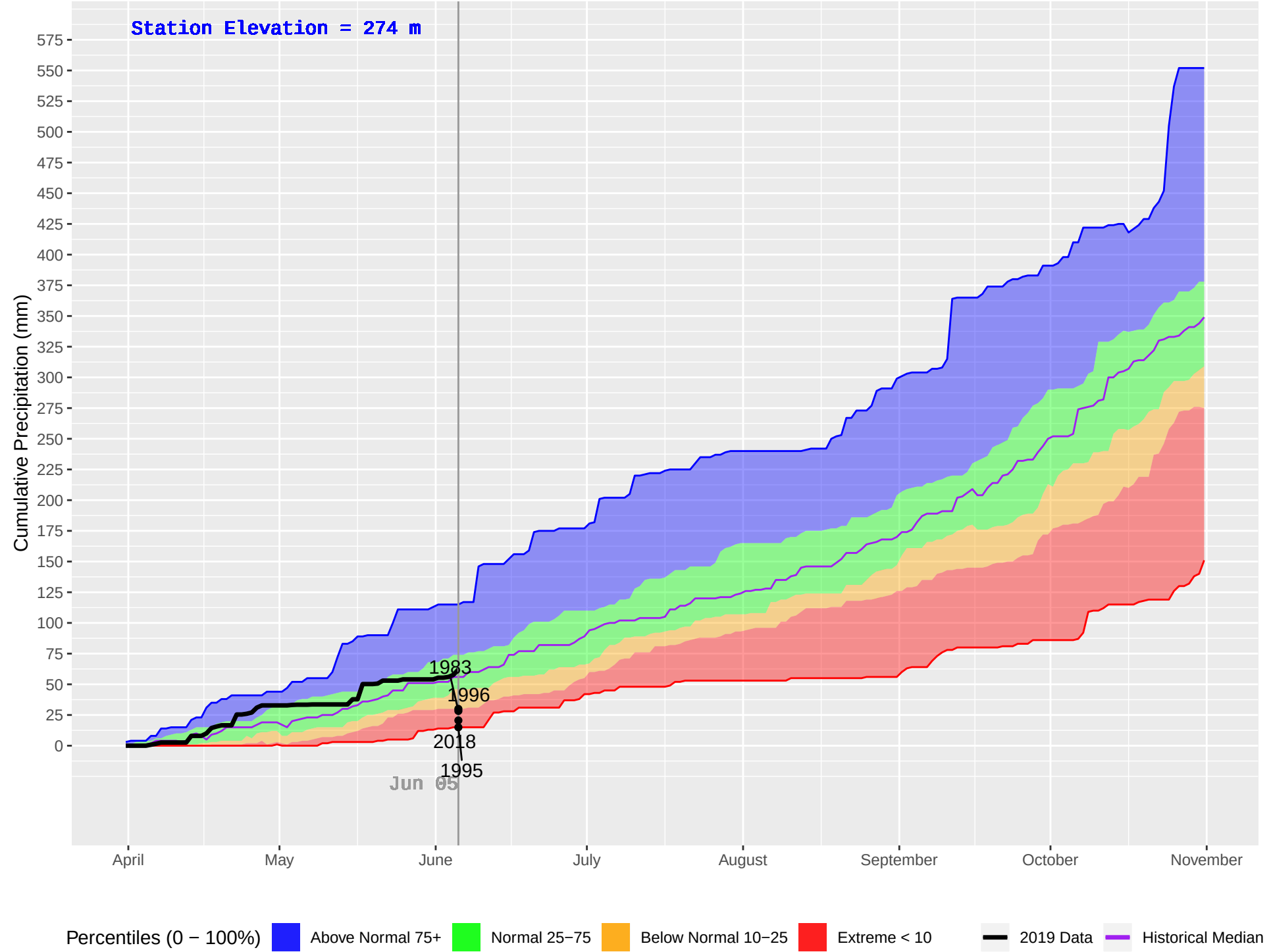
CEDARVALE (429) : Historical (1982–2018), Current (2019) Daily Cumulative Precipitation
