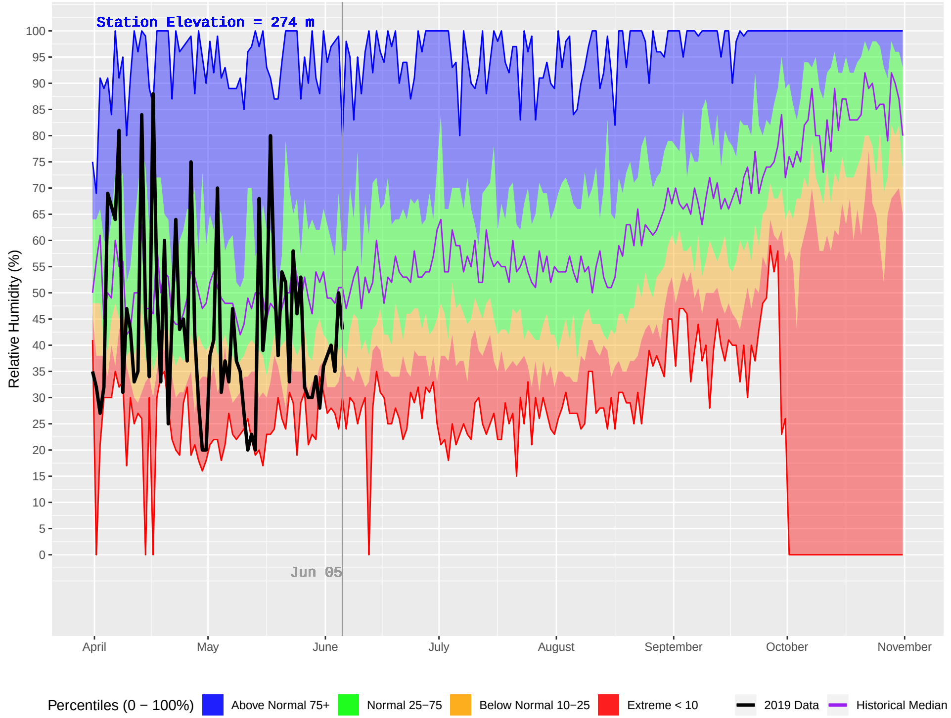
CEDARVALE (429) : Historical (1982–2018) and Current (2019) Daily Relative Humidity
