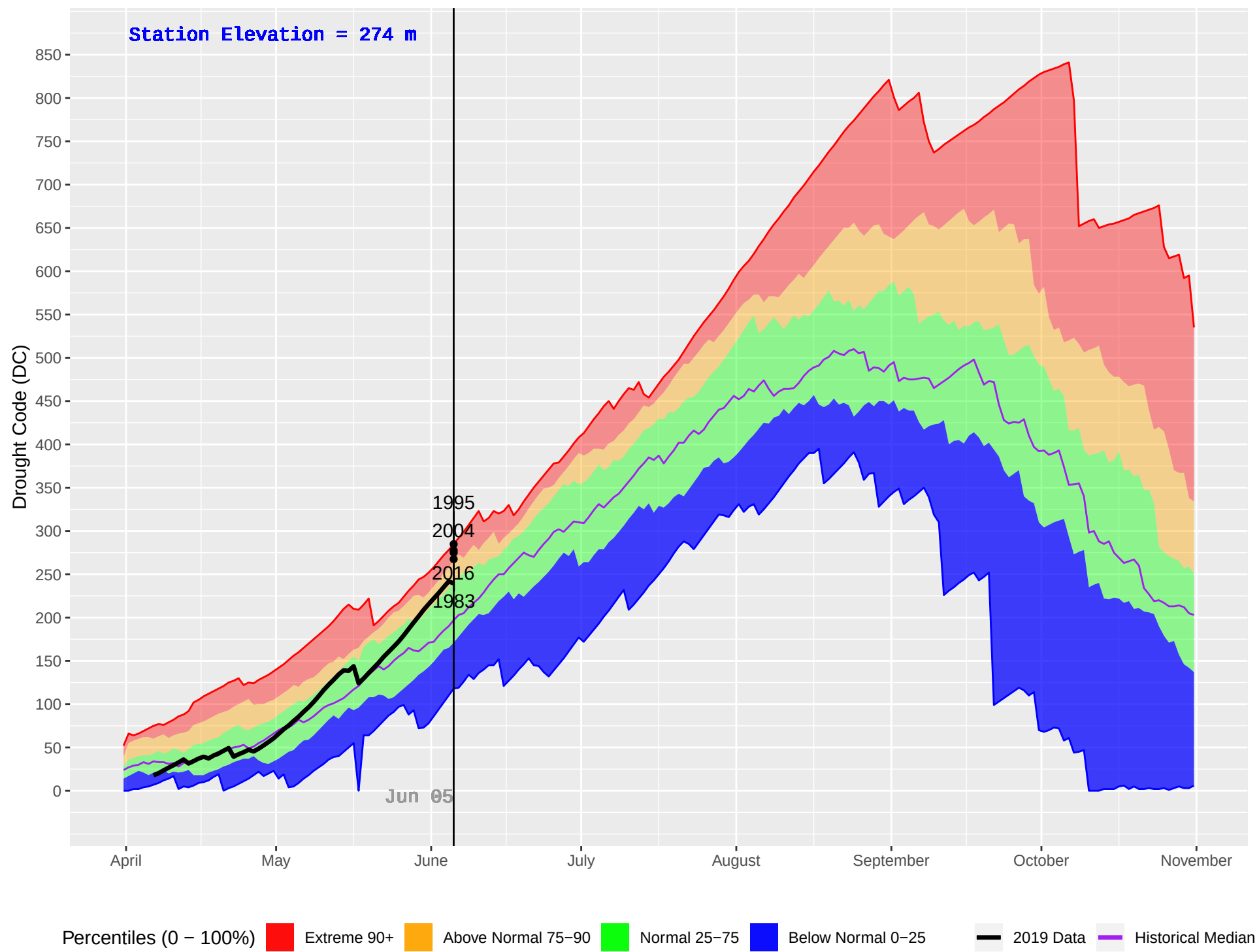
CEDARVALE (429) : Historical (1982–2018) and Current (2019) Daily Drought Code (DC)
