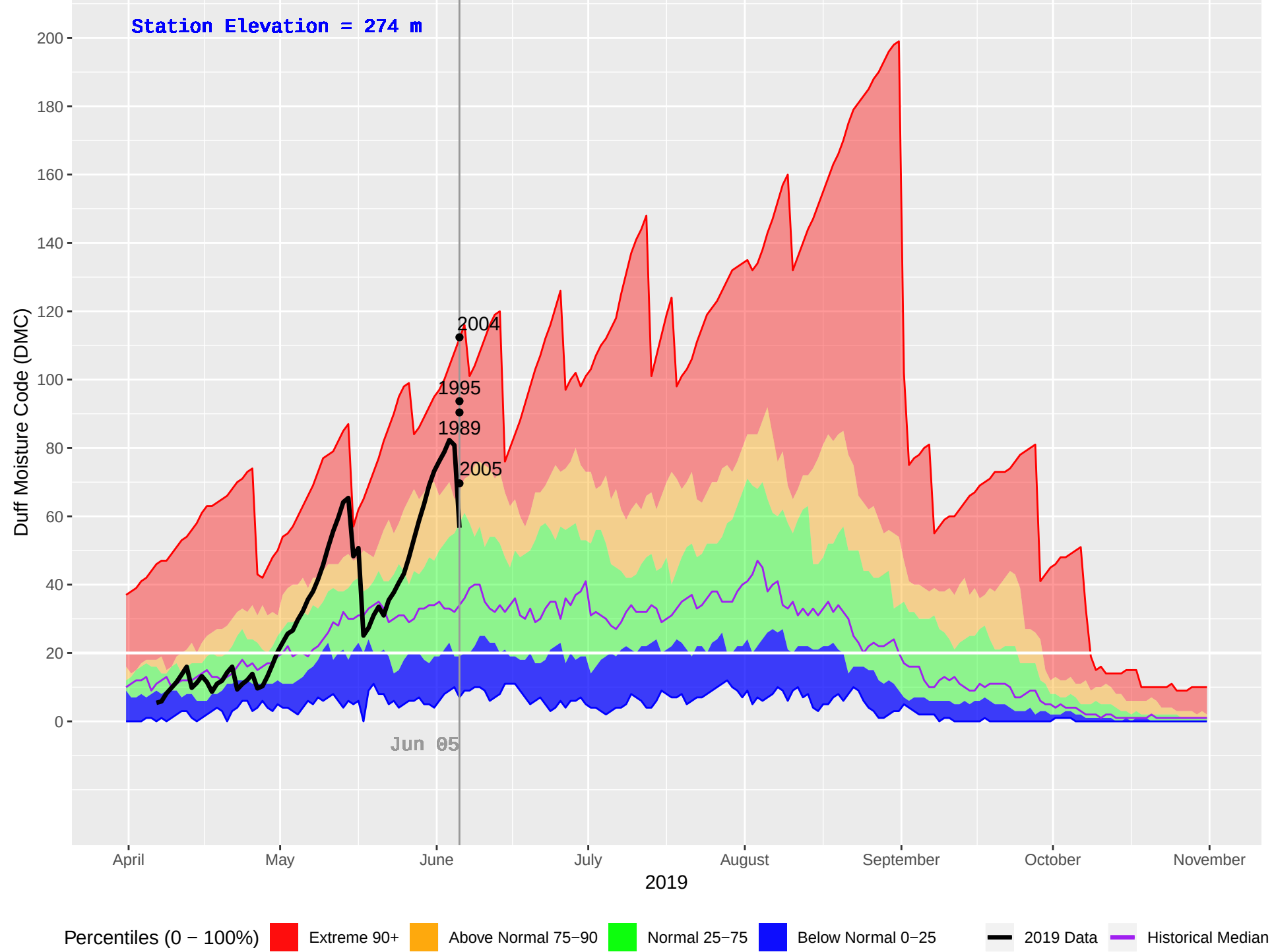
CEDARVALE (429) : Historical (1982–2018), Current (2019) Daily Duff Moisture Code (DMC)
