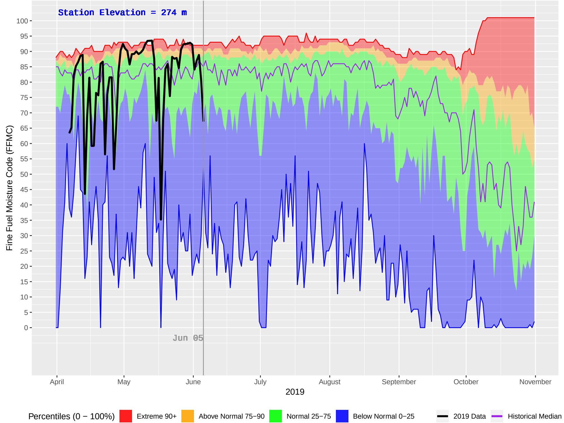
CEDARVALE (429) : Historical (1982–2018) and Current (2019) Daily Fine Fuel Moisture Code (FFMC)
